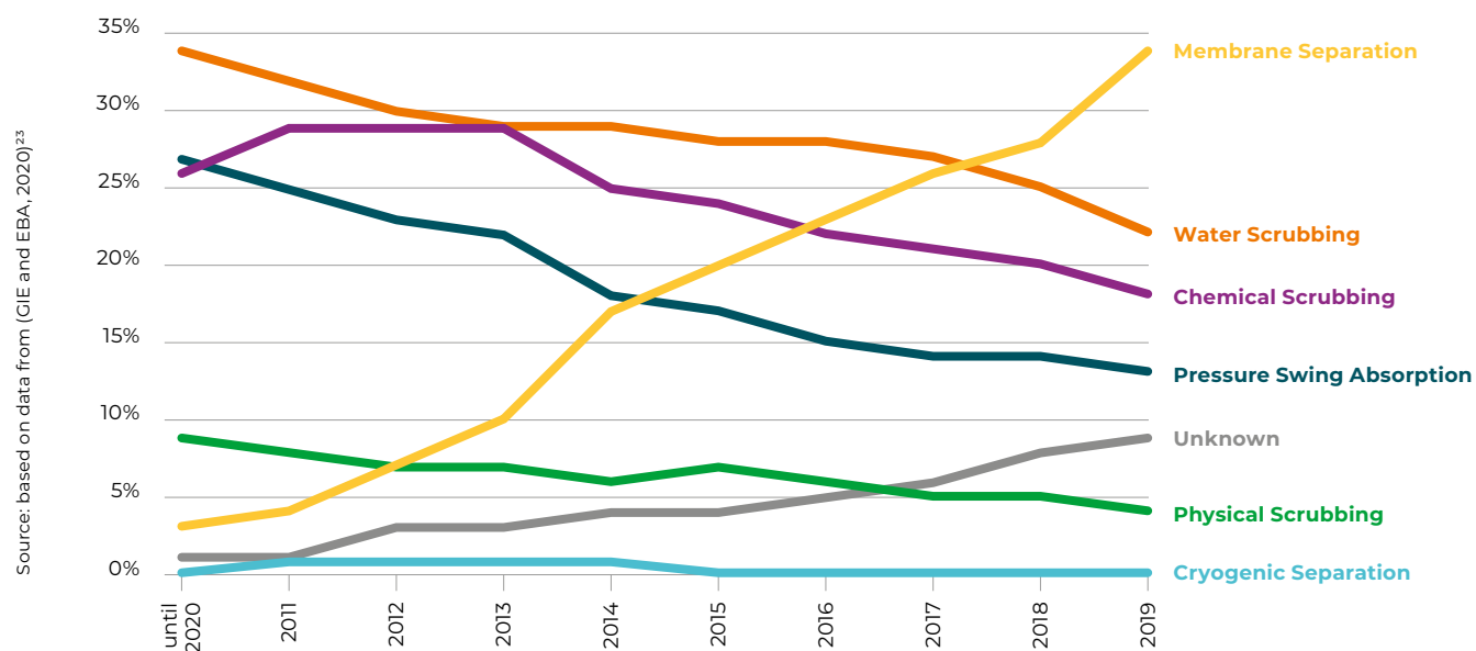
Figure 2.5. Cumulative change in biogas-biomethane upgrading techniques based on number of plants in Europe
