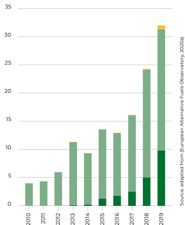
Figure 3.12. Cumulative number of heavy-duty trucks in the EU (thousands) on either electricity or gas (CNG/LNG/H 2 )
