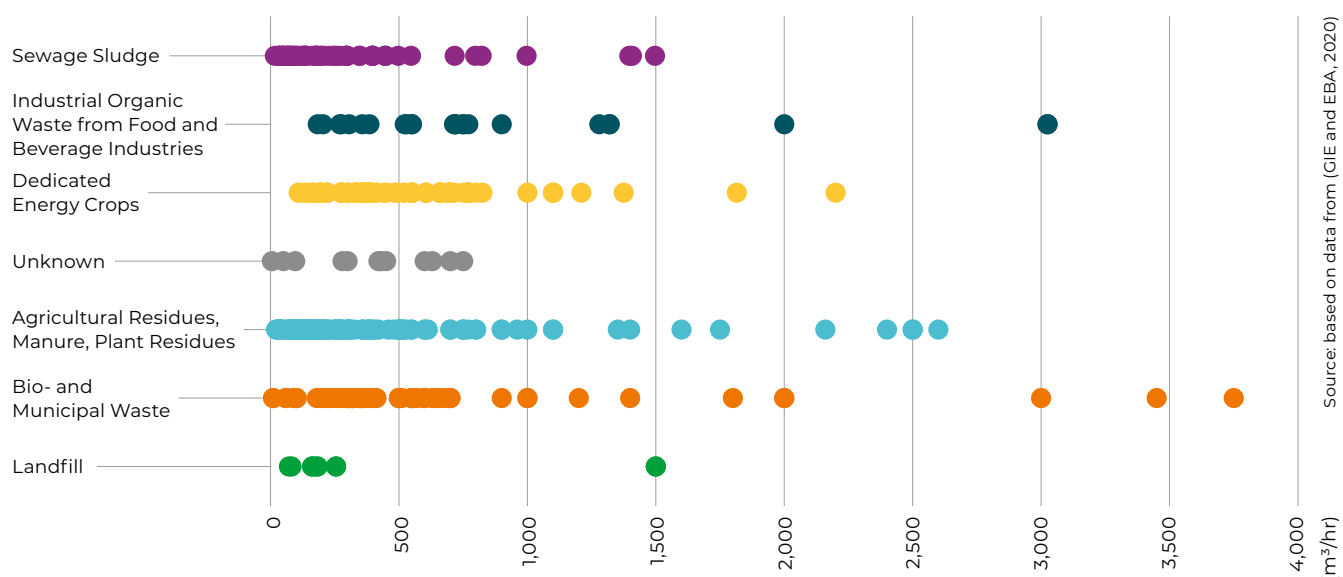
Figure 2.8. Biomethane production plant capacity ( \text{m}^3/\text{hr} ) vs. feedstock in the EU (cumulative numbers in 2019)
