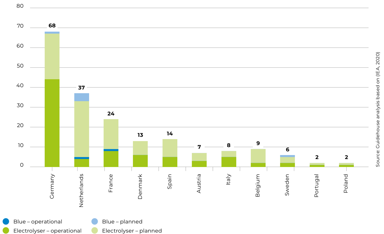
Figure 2.29. Number of electrolyser and blue hydrogen projects in the EU27 operational in 2020 and planned until 2030
