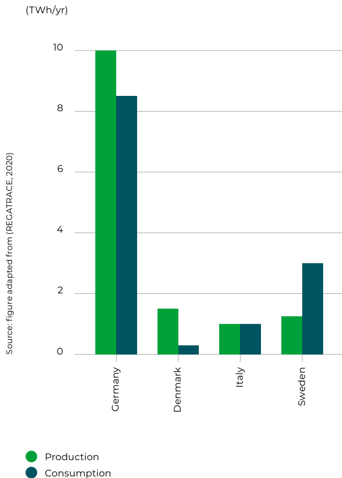
Figure 2.16. Estimated biomethane production and consumption for selected EU countries in 2018
