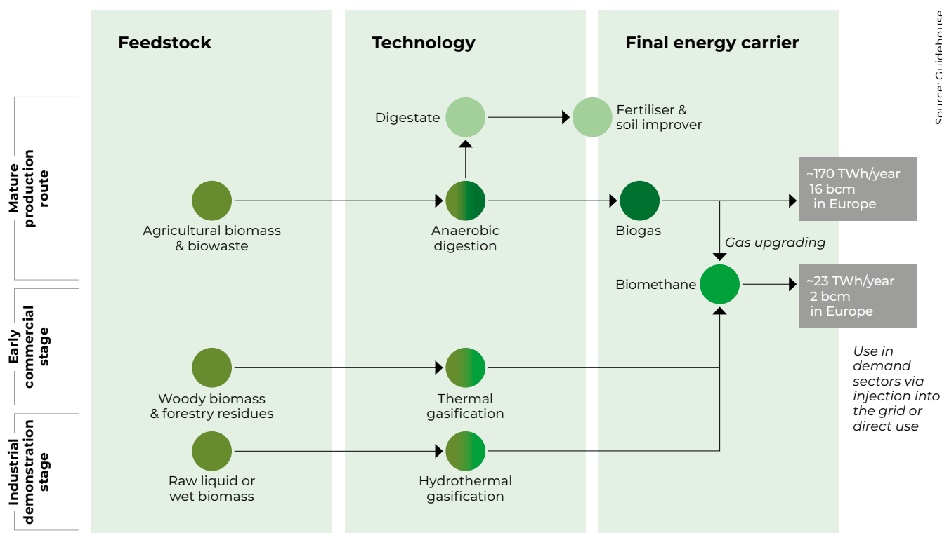
Figure 2.2. Overview of the two main production routes of biomethane
