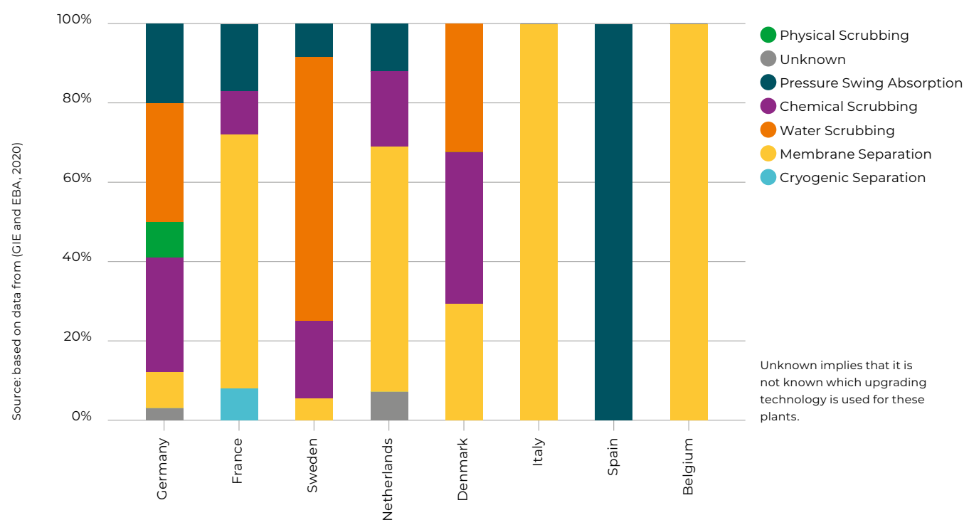
Figure 2.6. Indication of cumulative relative use of upgrading techniques based on number of plants in selected EU countries in 2019
