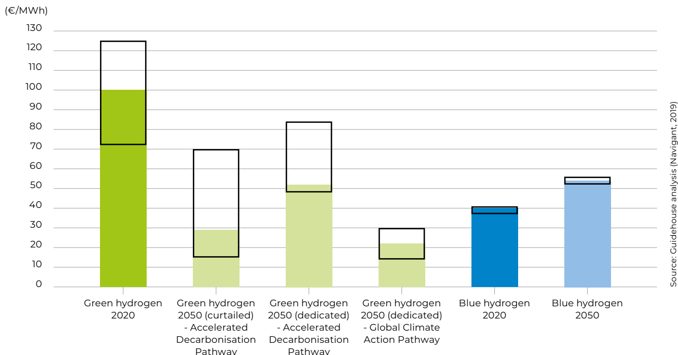
Figure 2.24. Hydrogen production cost estimates for 2020 and 2050
